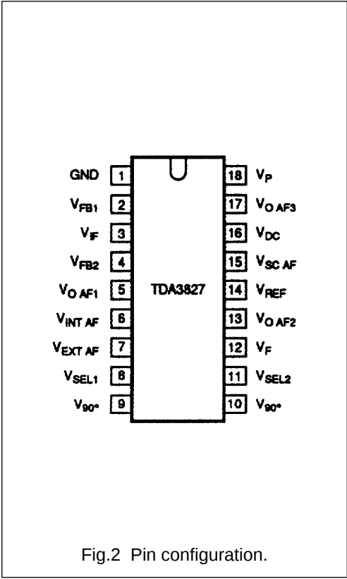
PIN CONFIGURATION
