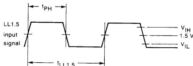
Fig. 5 LL1.5 timing waveform; 50/60 Hz picture frequency, parallel data transmission.
