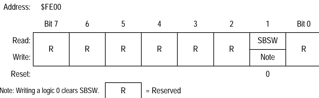
Figure 19-6. SIM Break Status Register (SBSR)
