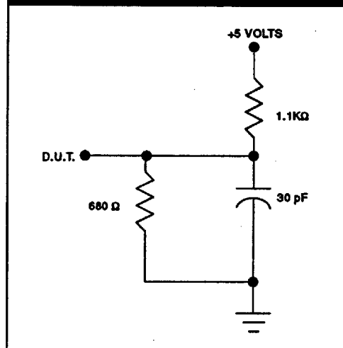
FIGURE 3: LOAD SCHEMATIC
