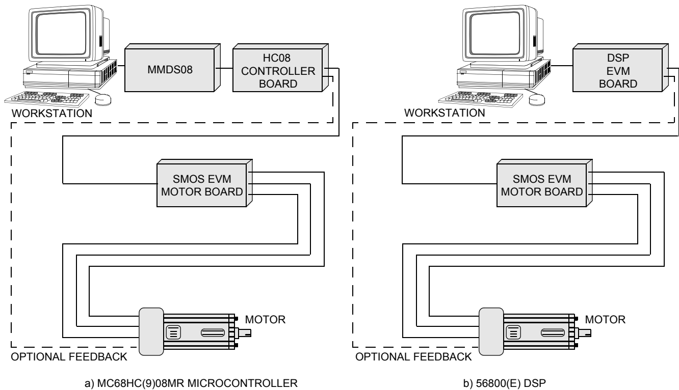
Figure 1-1 System Configurations
