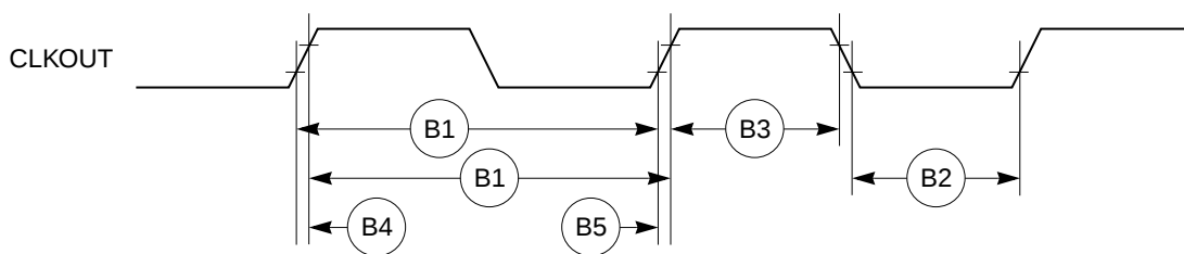
Figure 9-3. External Clock Timing
