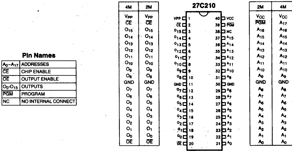
290193-2 Figure 2. DIP Pin Configuration
