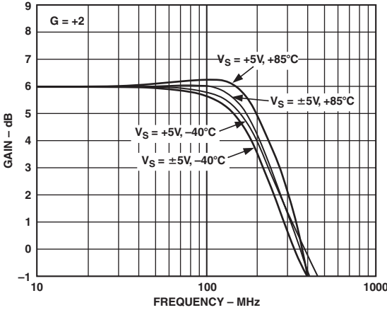
TPC 11. Small Signal Frequency Response over Temperature, V_S = +5 V, \pm 5 V
