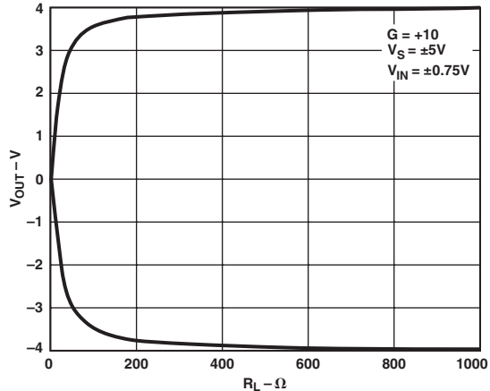
TPC 45. V_{OUT} Swing vs. R_{LOAD} , V_S = \pm 5V , G = +10 , V_{IN} = \pm 0.75V
