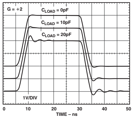
TPC 39. Large Signal Transient Response for Capacitive Load = 0\ \text{pF} , 10\ \text{pF} , and 20\ \text{pF}
