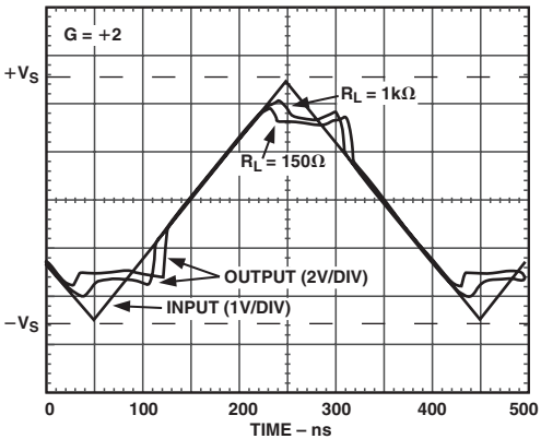
TPC 43. Output Overdrive Recovery, R_L = 1k\Omega , 150\Omega , V_{IN} = \pm 2.5V
