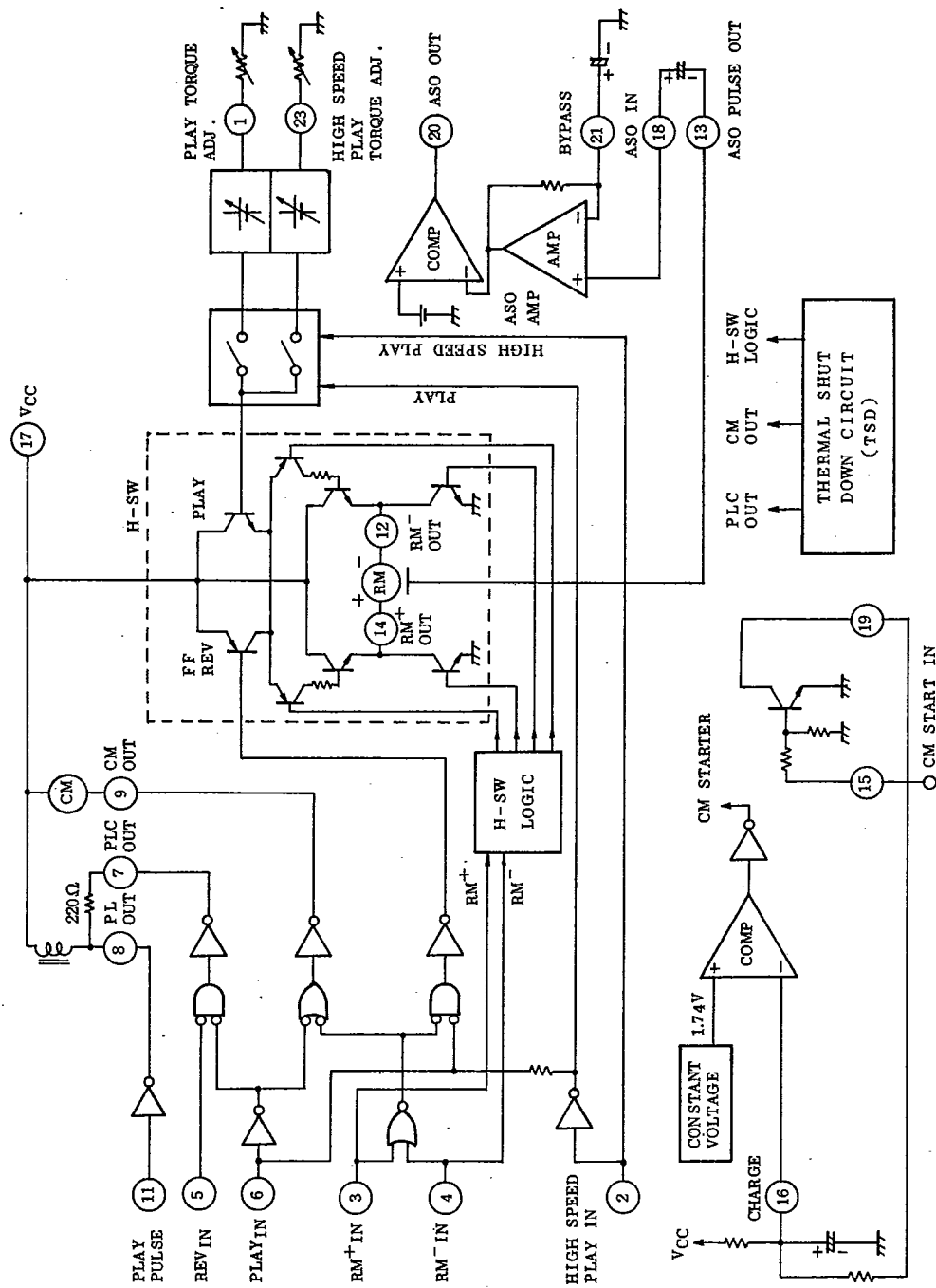
SYSTEM CHART
