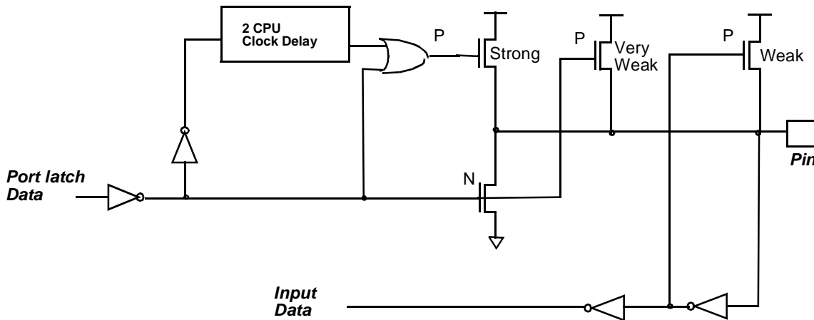
Figure 3. Quasi-Bi-directional Output
