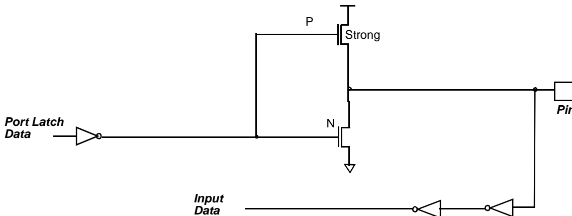
Figure 5. Push-pull Output
