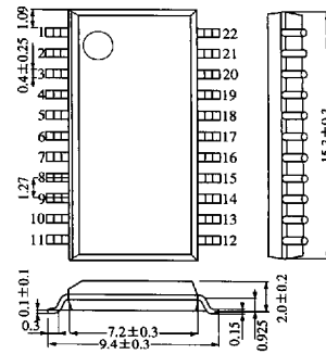
22-Pin PANAFLAT Package (SOP022-P-0375)
