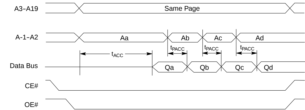
Figure 13. Page Read Timings
