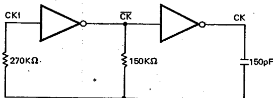
oscillator circuit
