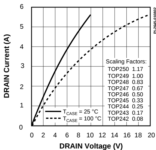
Figure 66. Output Characteristics.
