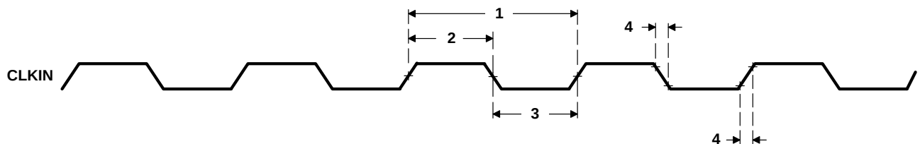
Figure 13. CLKIN Timing
