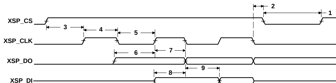
Figure 47. PCI Serial EEPROM Interface Timing
