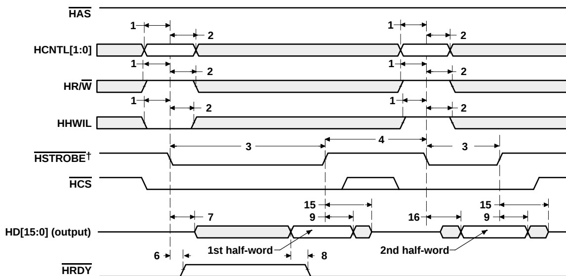
Figure 36. HPI16 Read Timing ( \overline{HAS} Not Used, Tied High)
