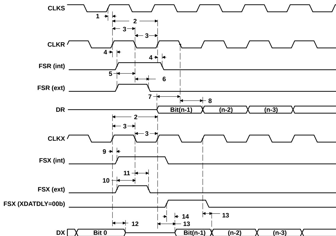
Figure 48. McBSP Timing
