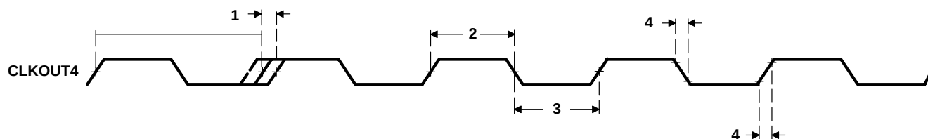
Figure 14. CLKOUT4 Timing
