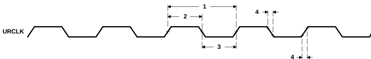
Figure 55. URCLK Timing
