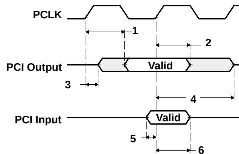
Figure 46. PCI Input/Output Timing
