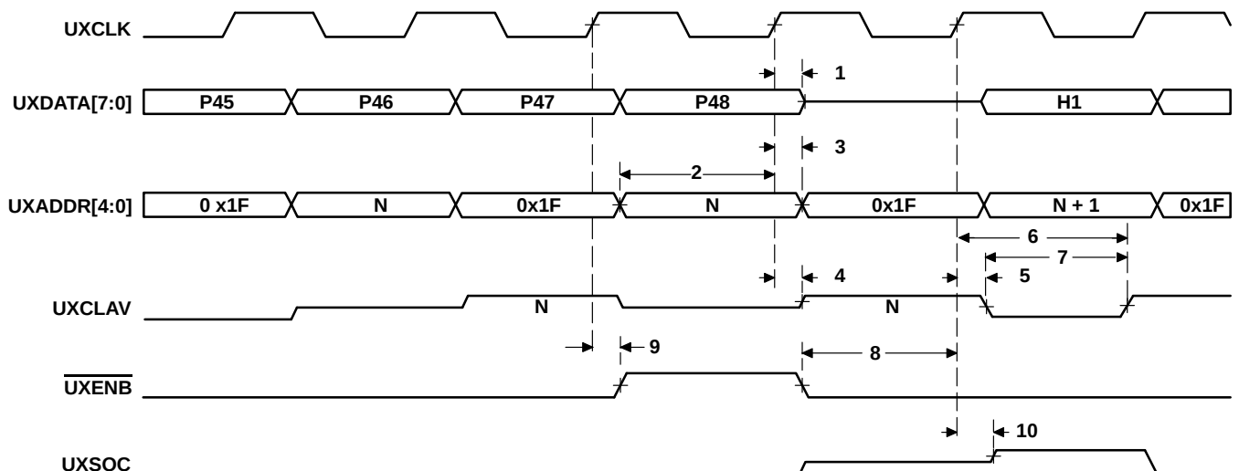
Figure 56. UTOPIA Slave Transmit Timing †
