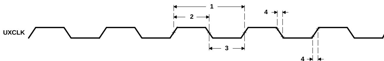
Figure 54. UXCLK Timing
