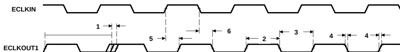
Figure 17. ECLKOUT1 Timing for EMIFA and EMIFB Modules
