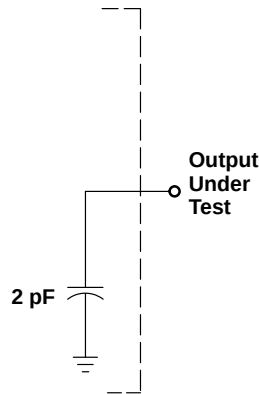
Figure 9. AC Timing Reference Circuit for AC Timing Measurements
