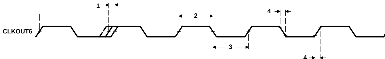
Figure 15. CLKOUT6 Timing
