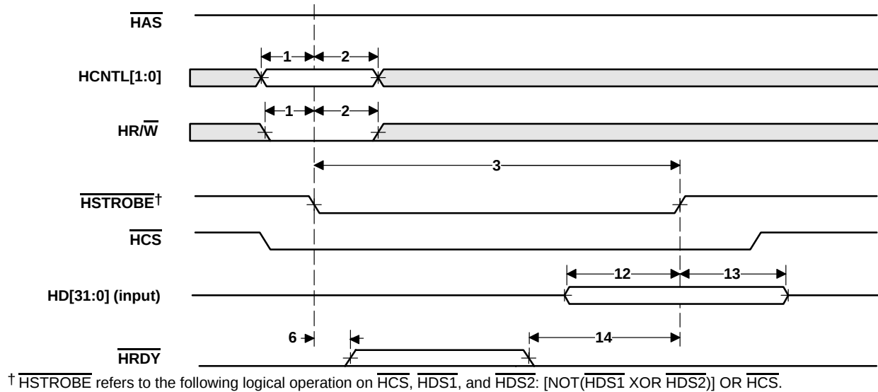
Figure 42. HPI32 Write Timing ( \overline{\text{HAS}} Not Used, Tied High)
