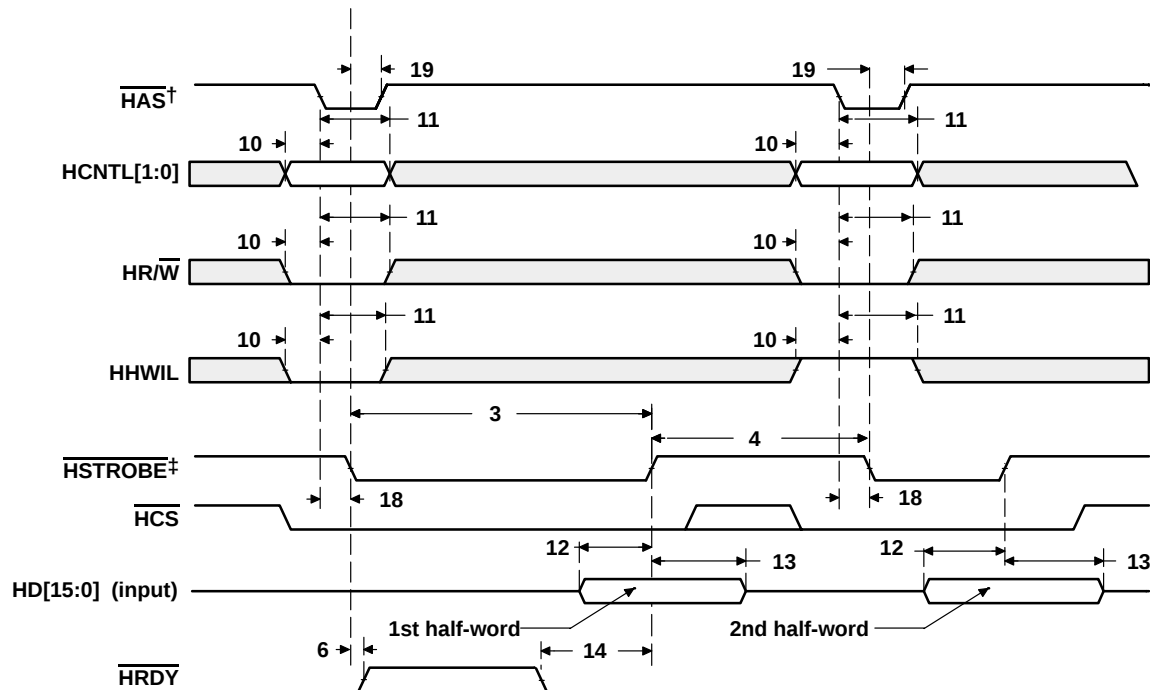
Figure 39. HPI16 Write Timing ( \overline{\text{HAS}} Used)
