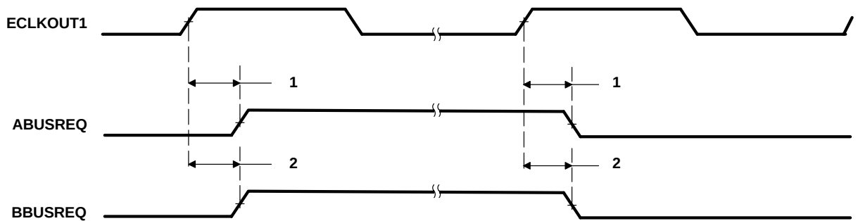
Figure 33. BUSREQ Timing for EMIFA and EMIFB
