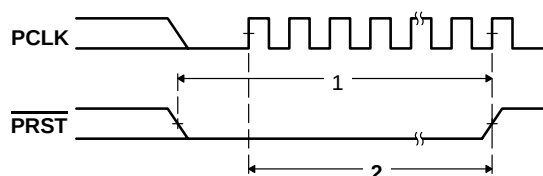
Figure 45. PCI Reset ( \overline{\text{PRST}} ) Timing
