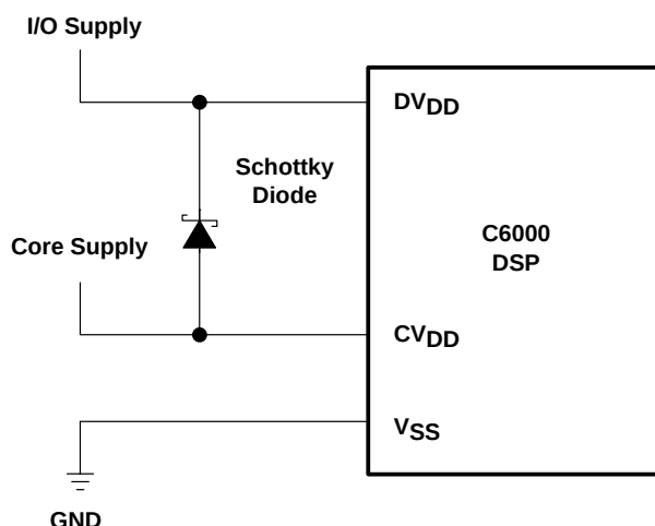
Figure 8. Schottky Diode Diagram
