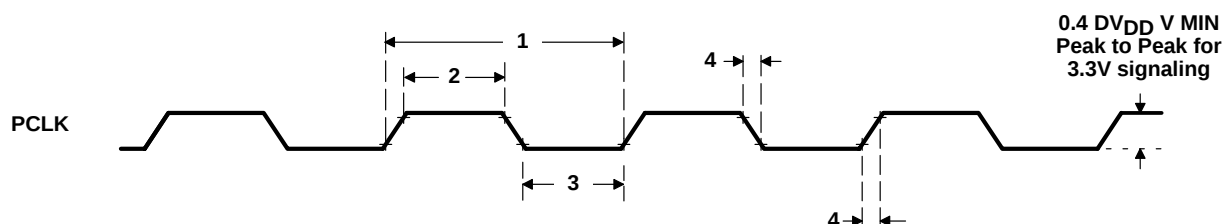
Figure 44. PCLK Timing
