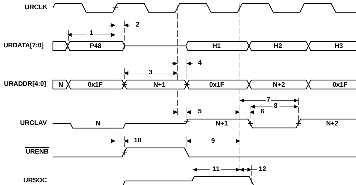
Figure 57. UTOPIA Slave Receive Timing†
