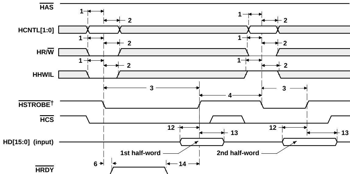
Figure 38. HPI16 Write Timing ( \overline{\text{HAS}} Not Used, Tied High)
