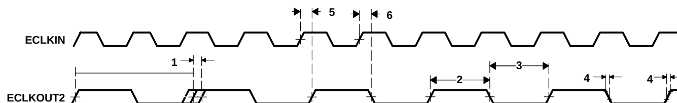
Figure 18. ECLKOUT2 Timing for the EMIFA and EMIFB Modules
