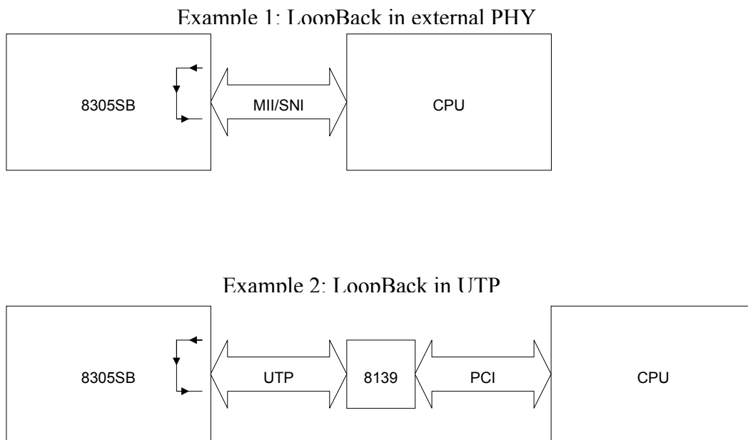
Figure 3: Port4 Loopback
