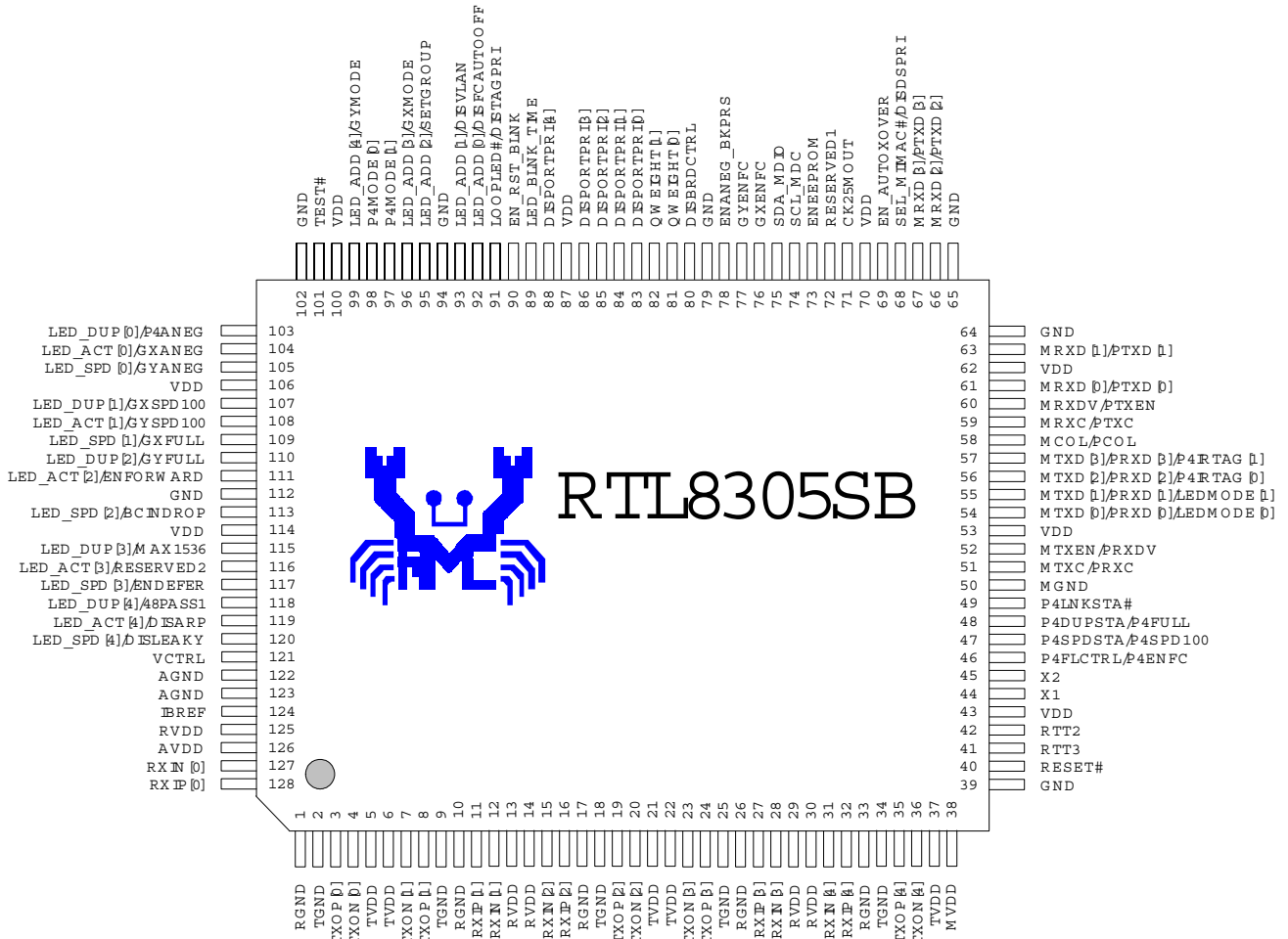
128 Pin RTL8305SB
