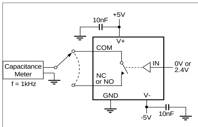
Figure 6. Channel-Off Capacitance
