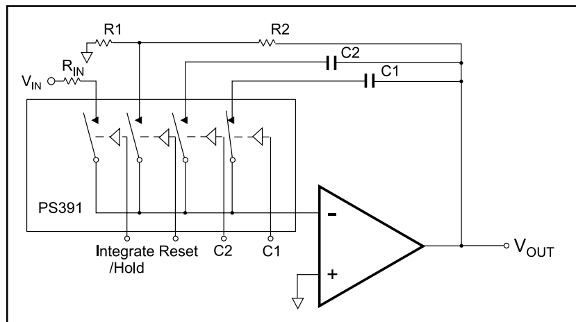
Figure 8. Programmable Integrator and Sample/Hold
