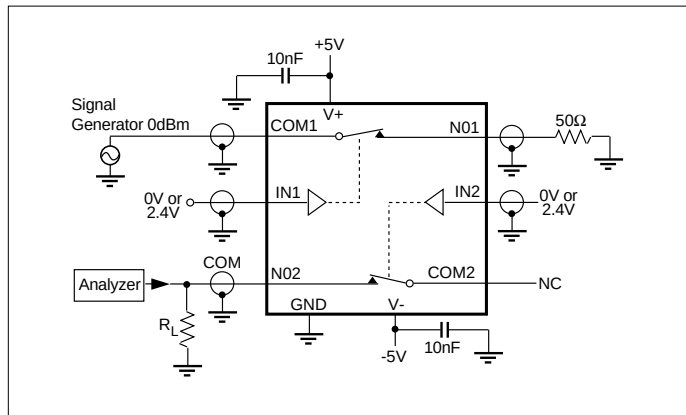
Figure 5. Crosstalk
