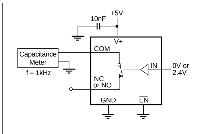
Figure 7. Channel-On Capacitance
