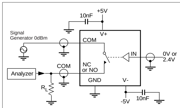
Figure 4. Off Isolation
