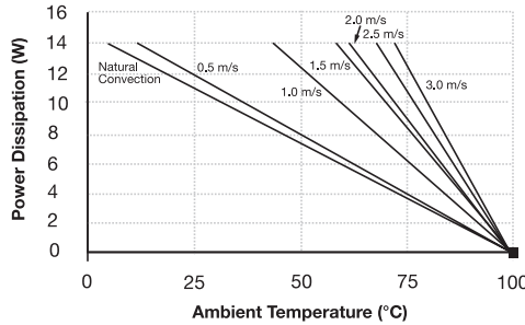
Allowable Power Dissipation vs. Ambient Temp. for 2.5V and 3.3V (PKJ 4719 PI, PKJ 4519 PI, PKJ 4319 PI, PKJ 4910 PI, PKJ 4610 PI, PKJ 4510 PI)
