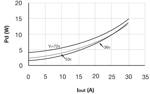
Power Loss vs. Output Current for 3.3V (PKJ 4910 PI, PKJ 4610 PI, PKJ 4510 PI)
