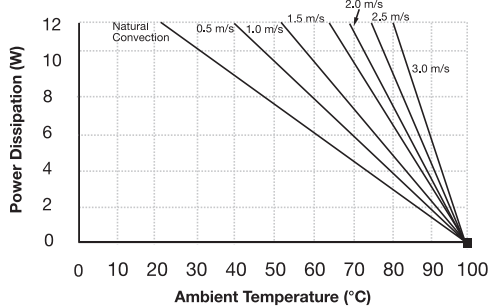
Allowable Power Dissipation vs. Ambient Temp. for 5V (PKJ 4711 PI, PKJ 4111 PI, PKJ 4111 API)
