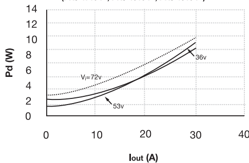
Power Loss vs. Output Current for 2.5V (PKJ 4719 PI, PKJ 4519 PI, PKJ 4319 PI)
