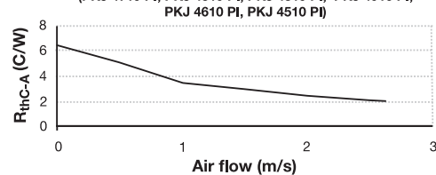
Case to Ambient Thermal Resistance for 2.5V and 3.3V (PKJ 4719 PI, PKJ 4519 PI, PKJ 4319 PI, PKJ 4910 PI, PKJ 4610 PI, PKJ 4510 PI)
