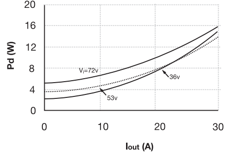
Power Loss vs. Output Current for 5V (PKJ 4711 PI, PKJ 4111 PI, PKJ 4111 API)
