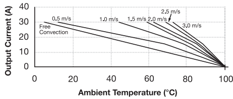
Output Current Derating (No heatsink) for 2.5V and 3.3V
