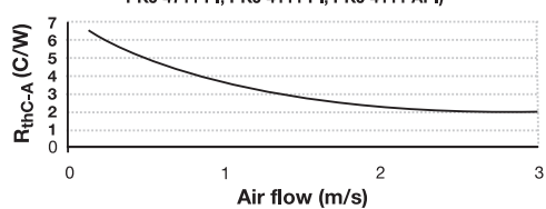
Case to Ambient Thermal Resistance for 5V (PKJ 4711 PI, PKJ 4111 PI, PKJ 4111 API)
