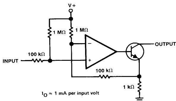
FIGURE 14. VOLTAGE-CONTROLLED CURRENT SINK
