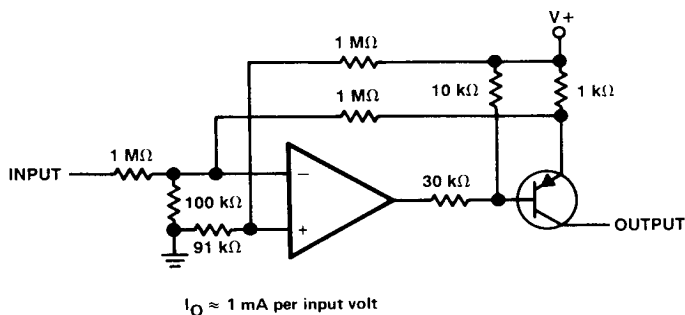
FIGURE 13. VOLTAGE-CONTROLLED CURRENT SOURCE
