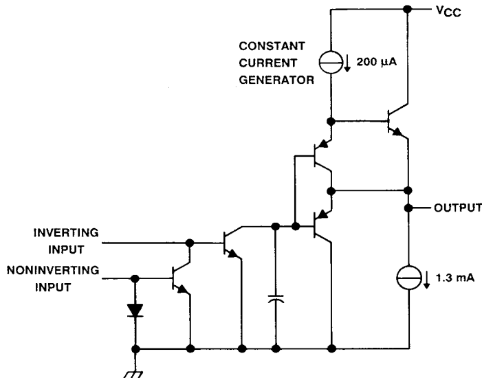
schematic (each amplifier)
