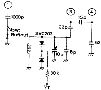
Unit (Resistance: Ω, Capacitance: F)
