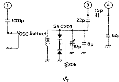
Unit (Resistance: Ω, Capacitance: F)
