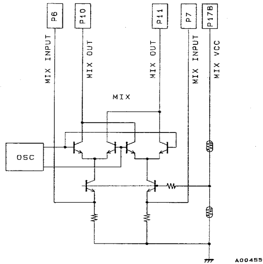
Figure 4 Mixer Circuit (Improved by 6.0 dBμ over previous products.)
