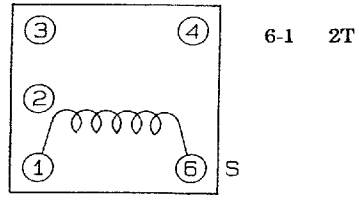
US band oscillator coil SA-278
