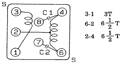
Mixer coil (for both bands) SA-266
