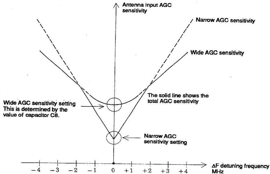
Figure 2 AGC Sensitivity Detuning Characteristics
