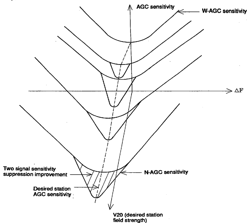
Figure 3 3D-AGC Sensitivity, \Delta f and V_{20} Characteristics
