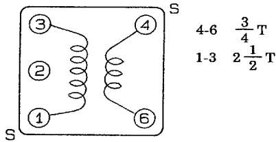
US band antenna coil SA-140 or SA-231
