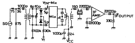
Unit (Resistance: \Omega , Capacitance: F)
