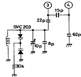
Unit (Resistance: \Omega , Capacitance: F)
