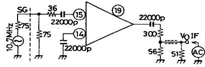
Unit (Resistance: \Omega , Capacitance: F)
