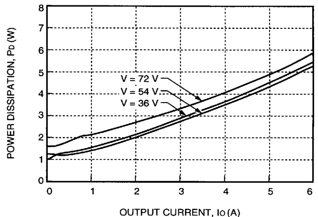
Figure 26. JW030D Power Dissipation vs. Output Current
