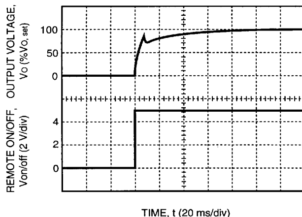
Figure 15. Typical Output Voltage Start-up when Signal Applied to Remote On/Off
