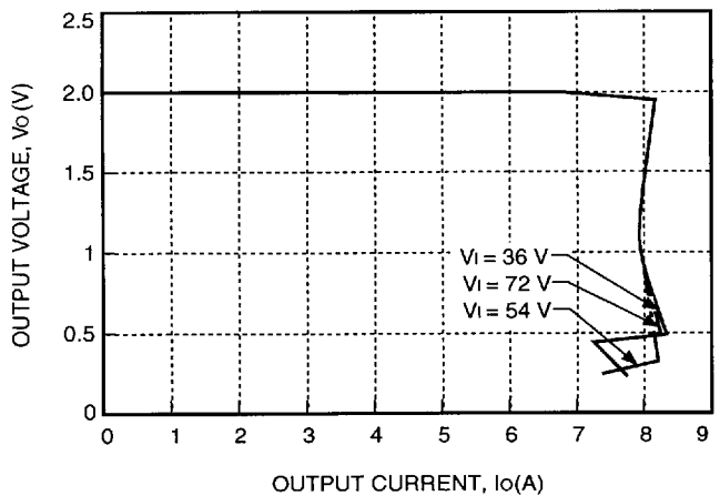
Figure 6. JW030D Typical Output Characteristics
