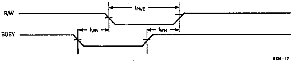
Write Timing with Busy Input ( M/\overline{S} =LOW)
