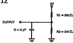
(c) Three-State Delay (Load 3)
