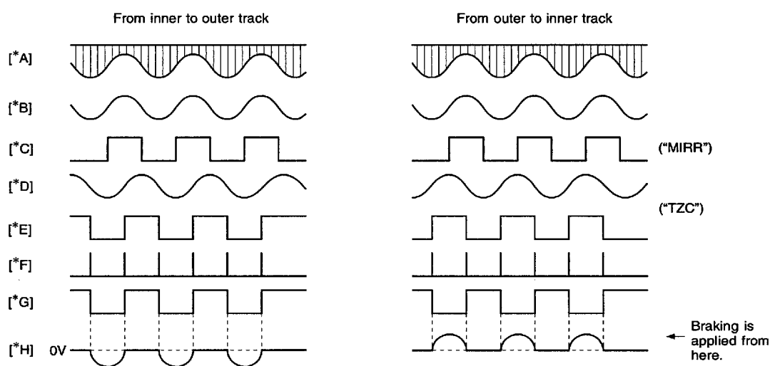
Fig. 7. Internal waveform
