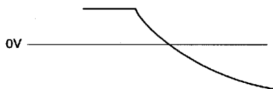
Fig. 1. Voltage at Pin 8 when FS1 goes from 0 → 1
