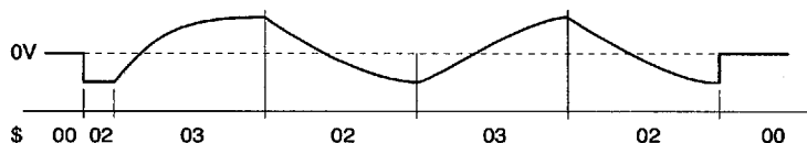
Fig. 2. Constructing the search voltage by alternating between $02 and $03. (Voltage at Pin 6)
