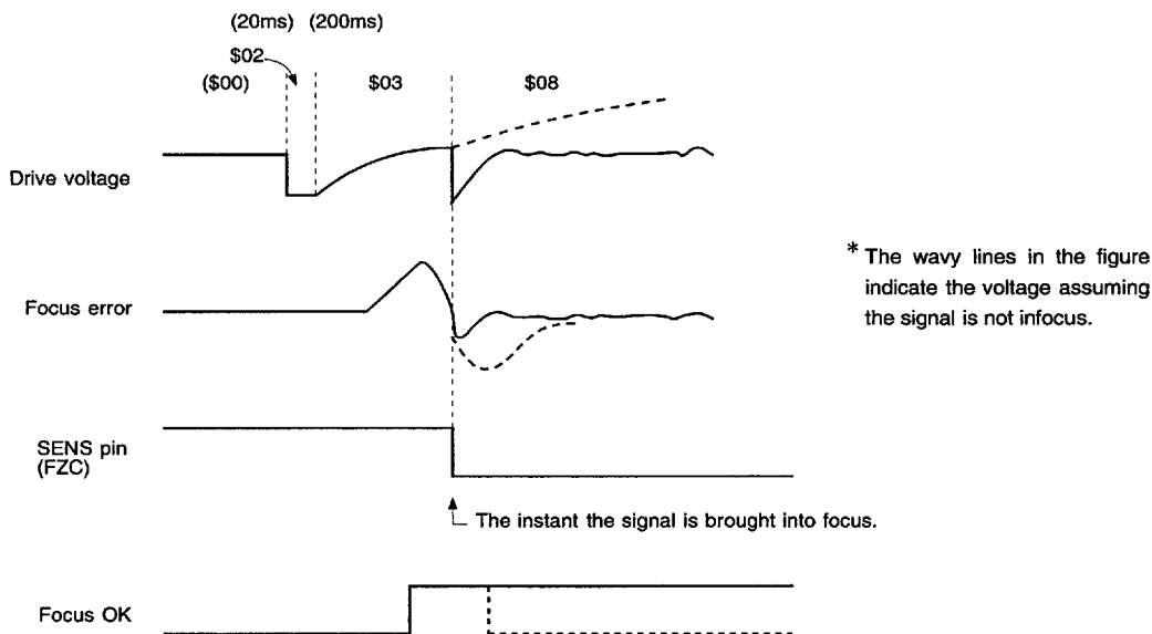
Fig. 4. Focus ON timing chart
