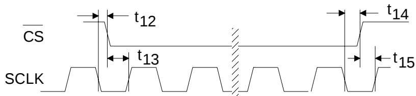
\overline{\text{CS}} with Continuous SCLK (Not to Scale)
