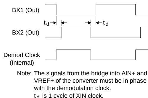
Figure 7. Internal Excitation Clock Phasing
