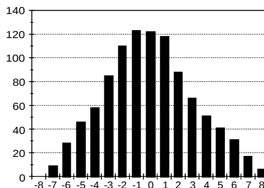
Figure 13. CS5520 Noise Histogram.
