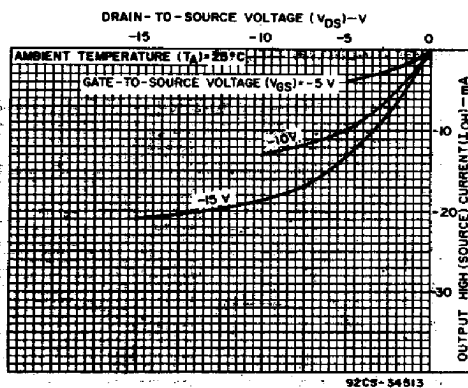
Fig. 2 - Typical output high (source) current characteristics.
