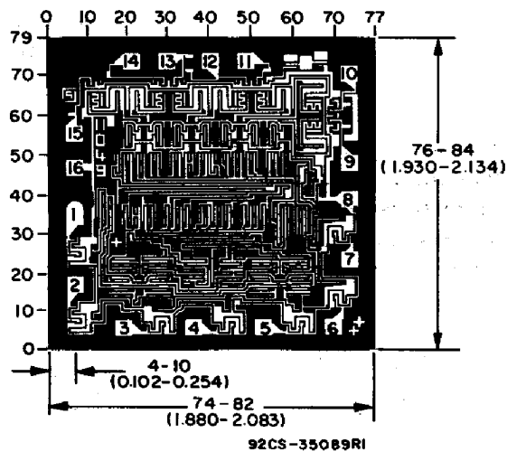
Dimensions and pad layout for CD4543BH.
