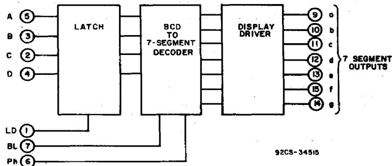
Fig. 4 - BCD-to-seven-segment latch/decoder/driver functional diagram.
