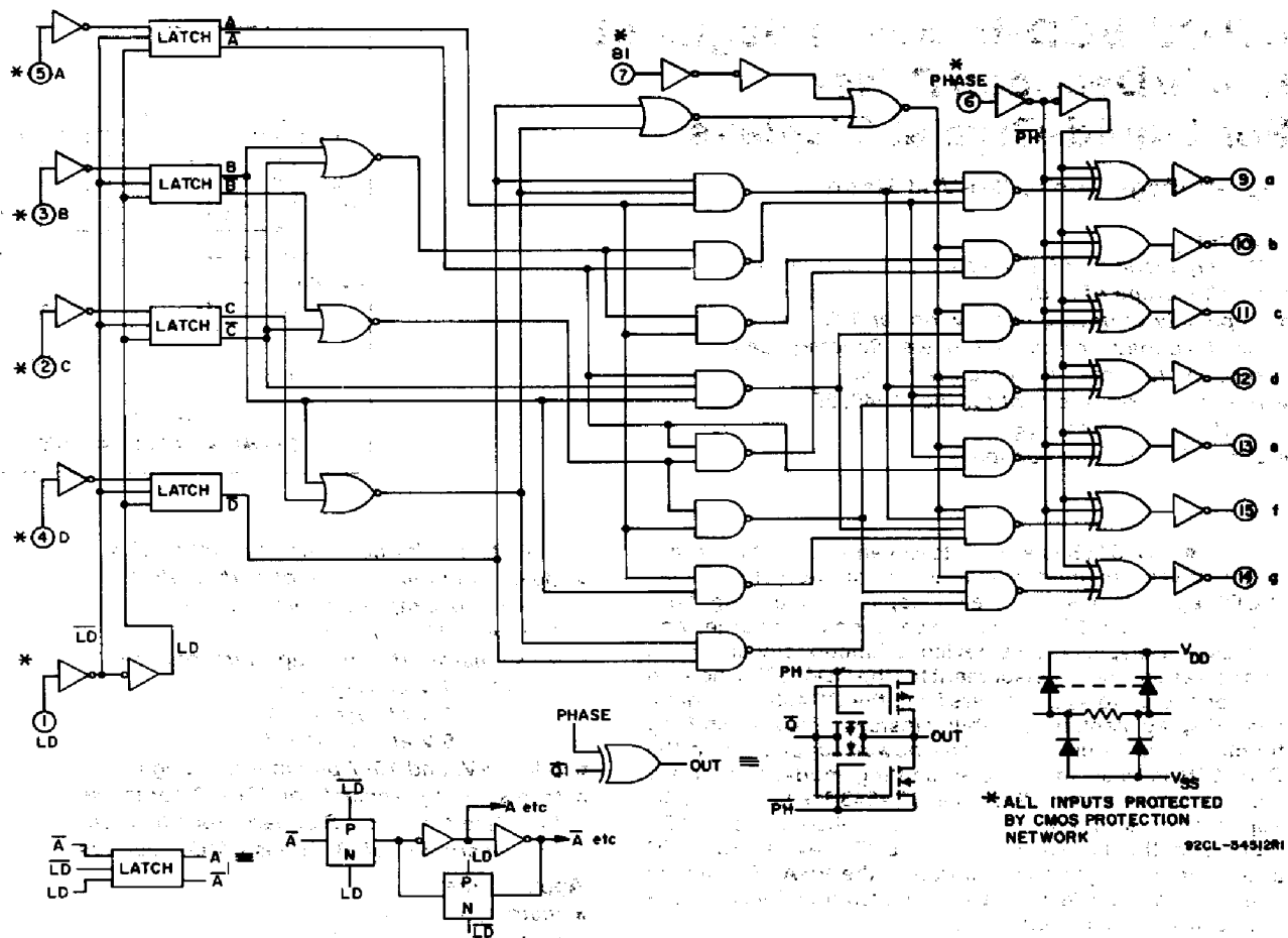
Fig. 1 - BCD-to-seven-segment latch/decoder/driver CD4543B logic circuit diagram.
