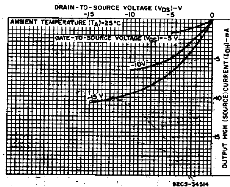
Fig. 3 - Minimum output high (source) current characteristics.
