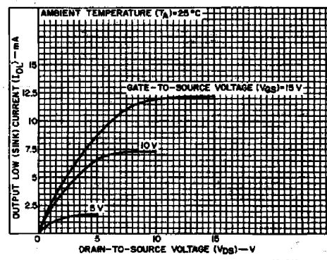
Fig. 6 - Minimum output low (sink) current characteristics.
