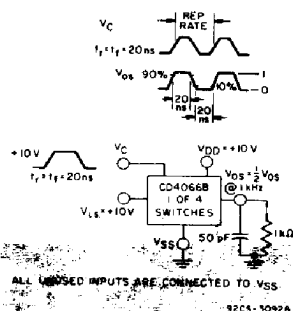
Fig. 15 - Maximum allowable control input repetition rate.
