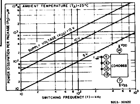
Fig. 9—Power dissipation per package vs. switching frequency.
