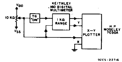
Fig. 7—Channel on-state resistance measurement circuit.
