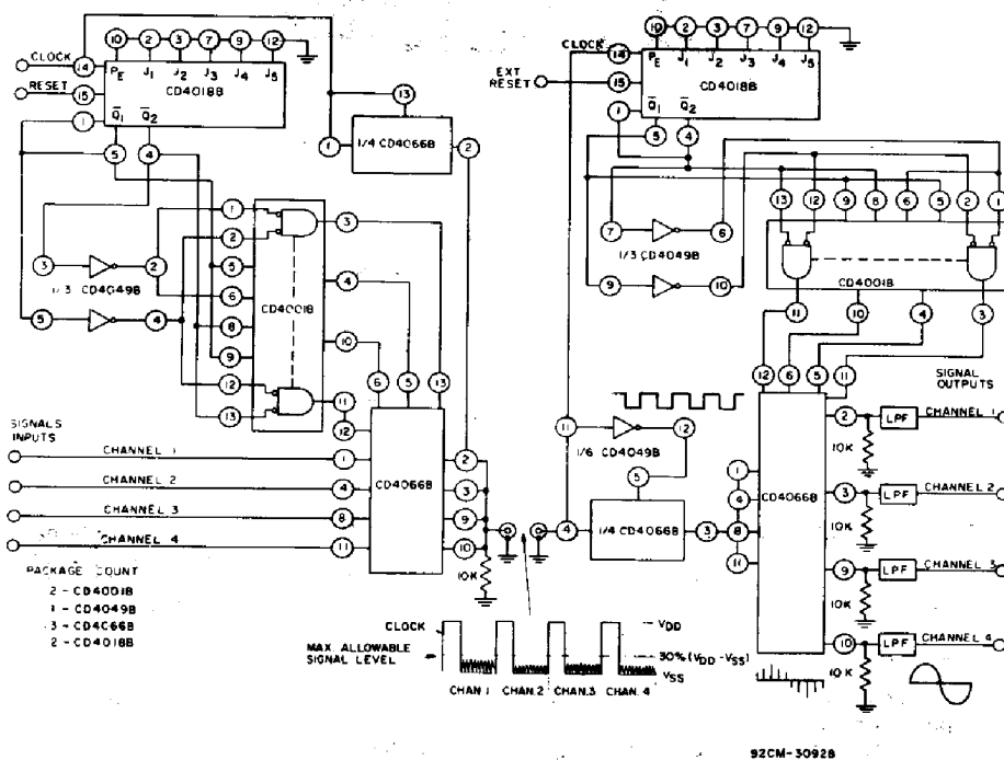
Fig. 17-- 4-channel PAM multiplex system diagram.
