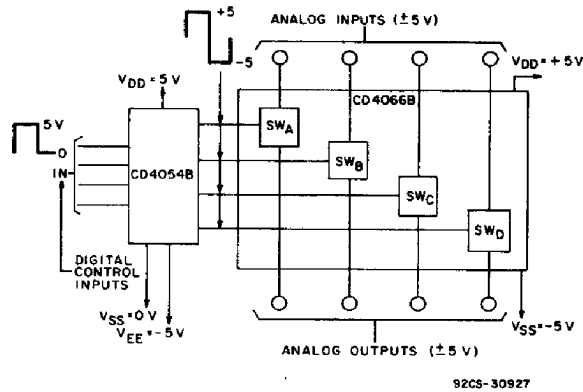
Fig. 18 — Bidirectional signal transmission via digital control logic.
