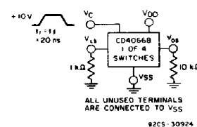
Fig. 13 – Crosstalk-control input to signal output.
