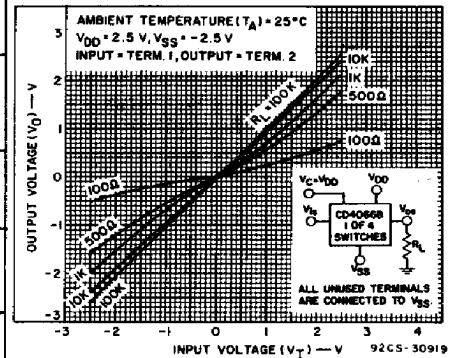
Fig. 8—Typical ON characteristics for 1 of 4 Channels.
