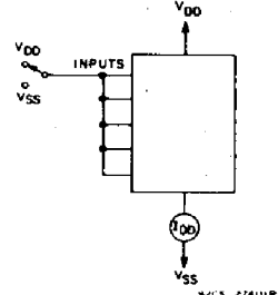
Fig. 12 — Quiescent device current test circuit.
