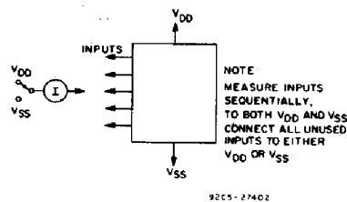
Fig. 9 — Input current test circuit.
