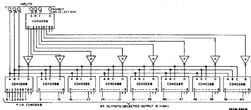
Fig. 15 — 6-bit binary to 1-of-64 address decoder.
