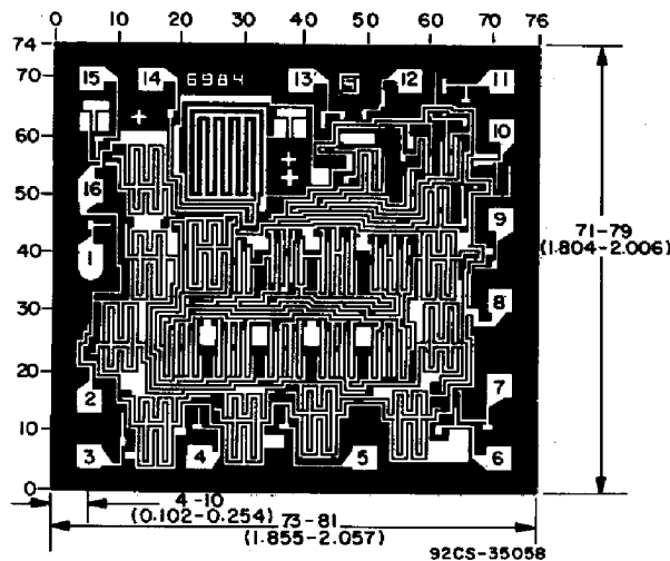
CD4028BH DIMENSIONS AND PAD LAYOUT
