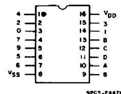
Top View TERMINAL DIAGRAM
