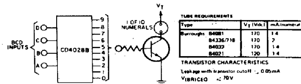
Fig. 14 — Neon readout (Nixie Tube ^ ) display application.
