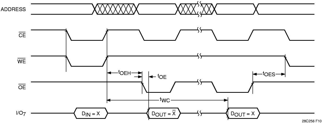
Figure 7. \overline{\text{DATA}} Polling
