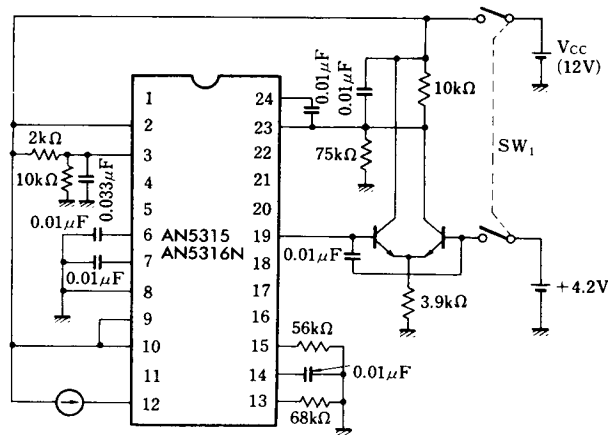
Test Circuit 1 ( I_{tot} , V_{19-8} , V_{20, 21, 22-8} )
