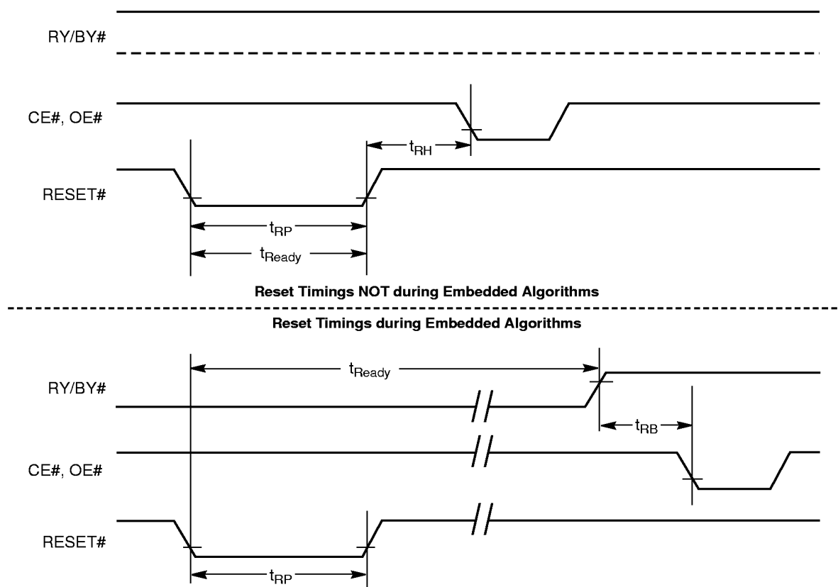
Figure 14. RESET# Timings
