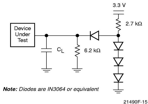
Figure 11. Test Setup
