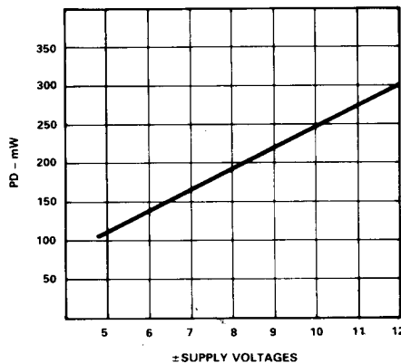
Power Dissipation vs. Supply Voltages
