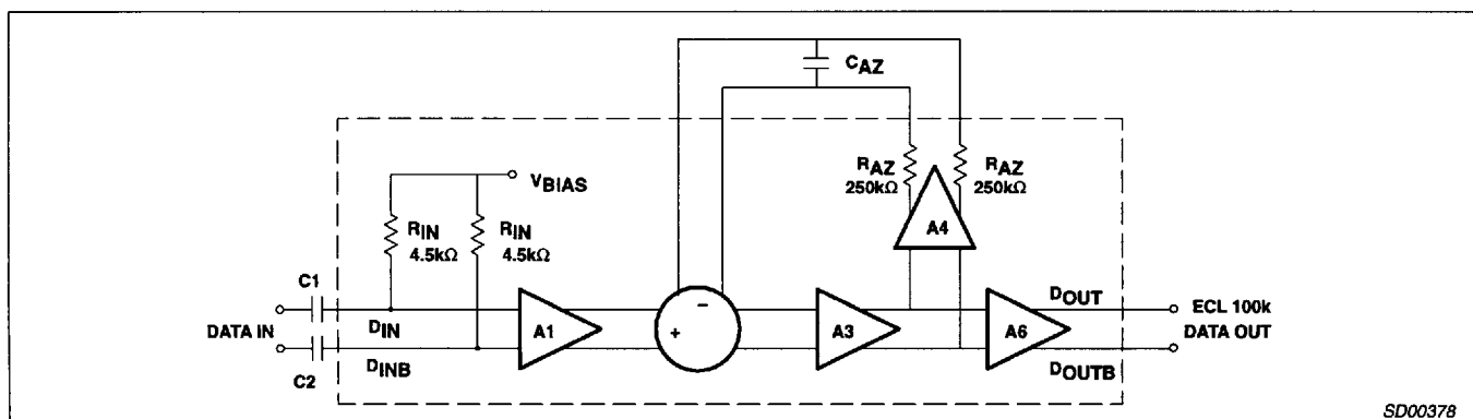
Figure 1. NE5224 Forward Gain Path Including Auto-Zero
