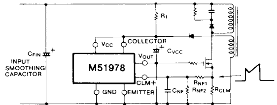
Fig. 24 Peripheral circuit diagram of CLM + terminal
