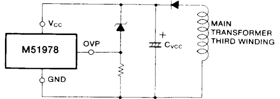
Fig. 23 OVP setting method using the induced third winding voltage on fly back system
