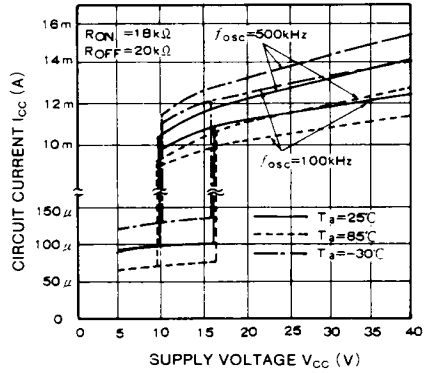
CIRCUIT CURRENT VS. SUPPLY VOLTAGE (NORMAL OPERATION)
