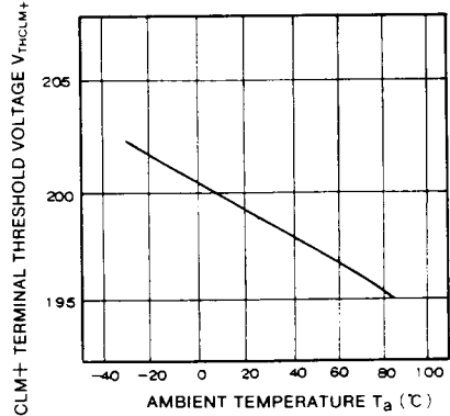
CLM+ TERMINAL THRESHOLD VOLTAGE VS. AMBIENT TEMPERATURE
