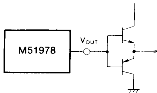
Fig. 35 Output buffer circuit diagram
