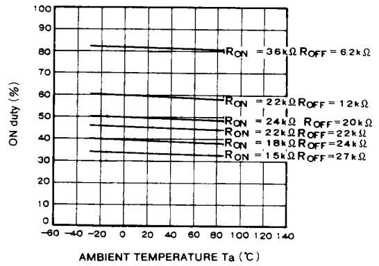
ON duty VS. AMBIENT TEMPERATURE
