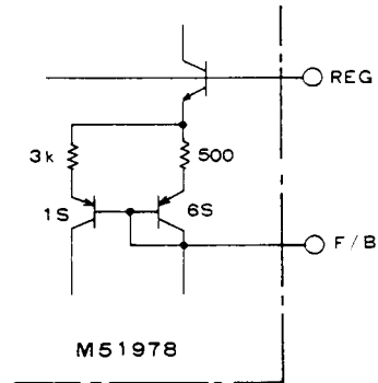
Fig. 27 Relationship between REG terminal and F/B terminal
