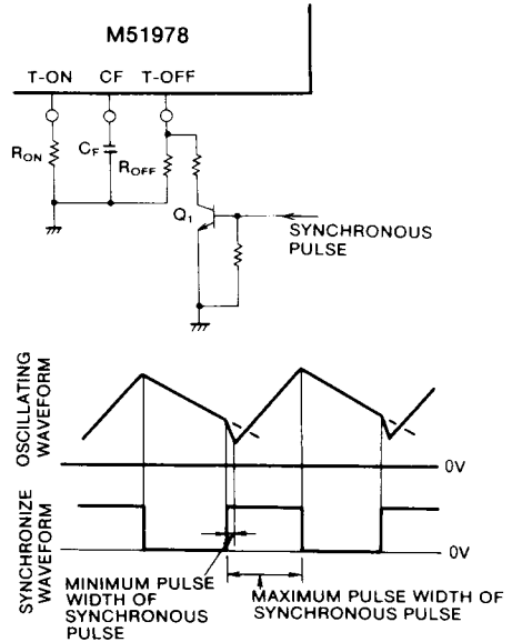
Fig. 39 How to synchronize with external circuit
