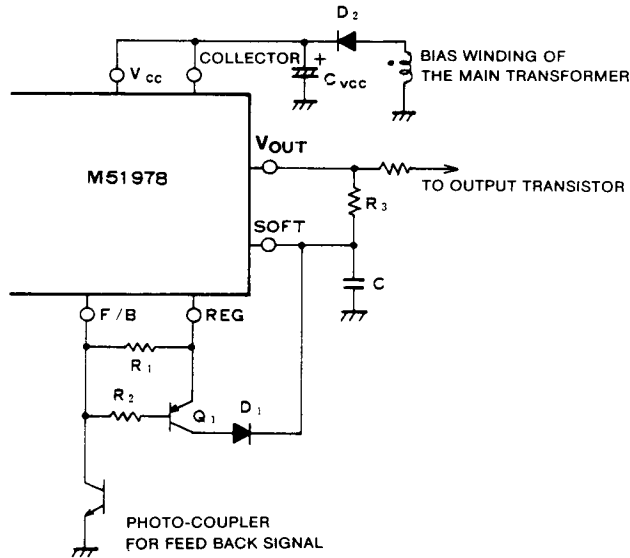
Fig. 28 Circuit to lower frequency during over current
