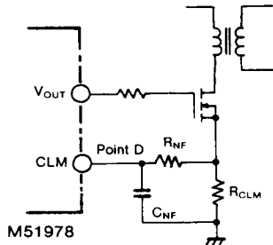
Fig.12 Connection diagram of current limit circuit
