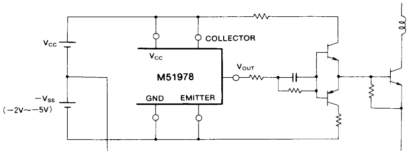
Fig. 40 Driver circuit diagram (1) for bipolar transistor
