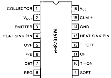
Outline 16P2N
