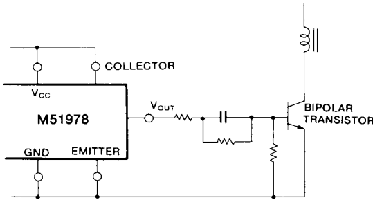
Fig. 41 Driver circuit diagram (2) for small bipolar transistor
