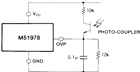
Fig. 21 Peripheral circuit of OVP terminal
