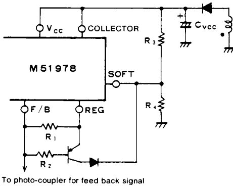
Fig. 32 Circuit to lower the frequency during the over current in the fly back system
