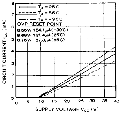
CIRCUIT CURRENT VS. SUPPLY VOLTAGE (OVP OPERATION)
