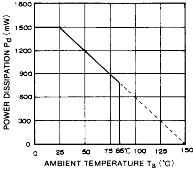
THERMAL DERATING (MAXIMUM RATING)
