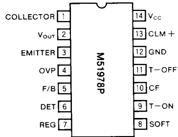
Outline 14P4
