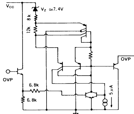
Fig.15 Detail diadram of OVP circuit
