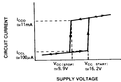
Fig.3 Start-up current vs. supply voltage
