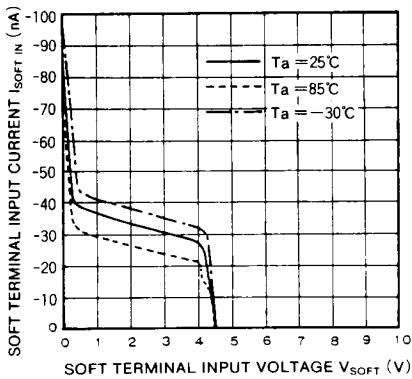
SOFT TERMINAL INPUT CURRENT VS. INPUT VOLTAGE
