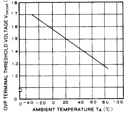
OVP TERMINAL THRESHOLD VOLTAGE VS. AMBIENT TEMPERATURE
