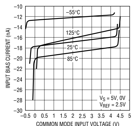
Input Bias Current vs Common Mode Input Voltage
