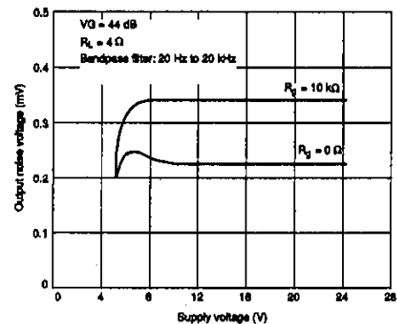
Noise voltage vs. supply voltage
