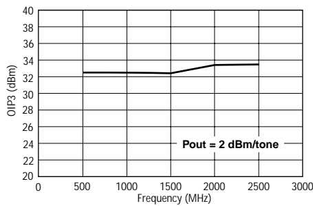
OIP3 vs. Frequency
