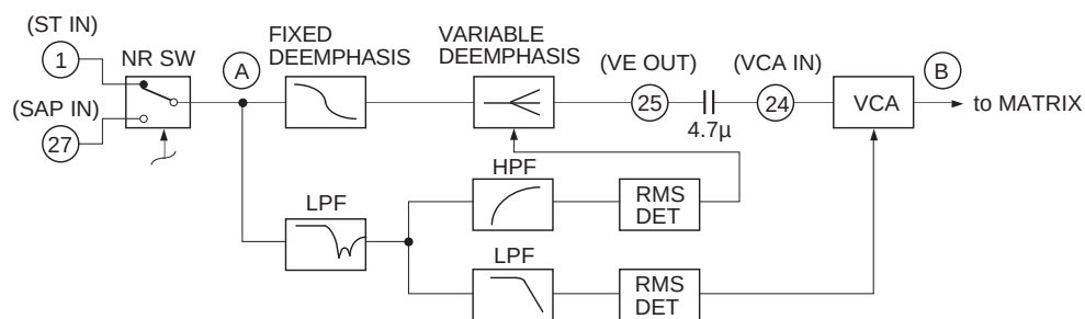
Fig 4. dbx-TV block
