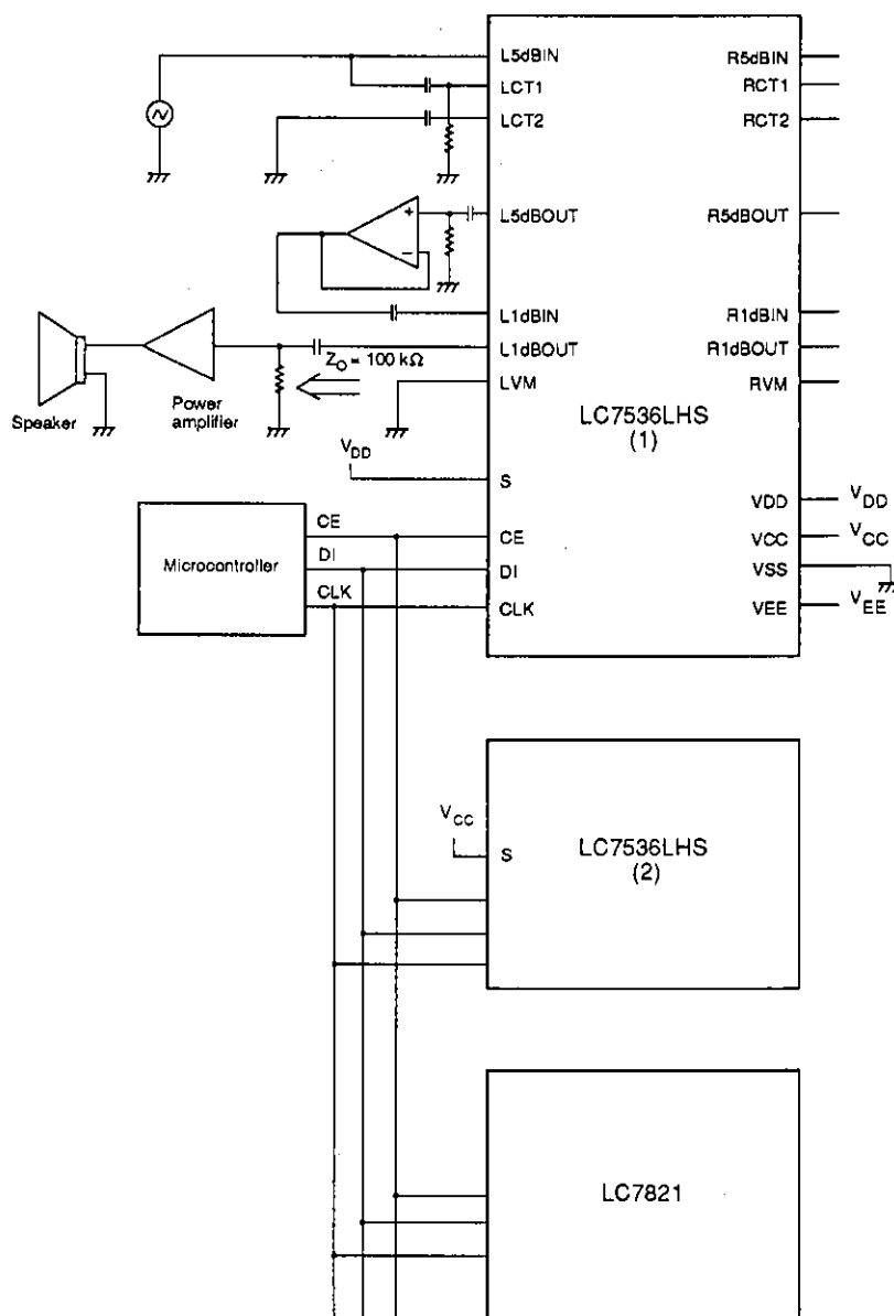
Figure 2. Typical application
