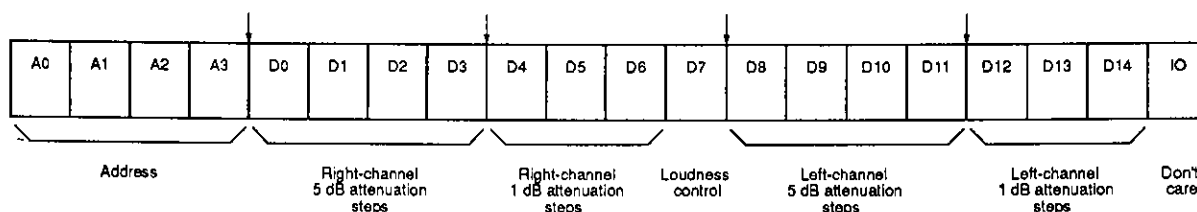
Figure 1. Data format
