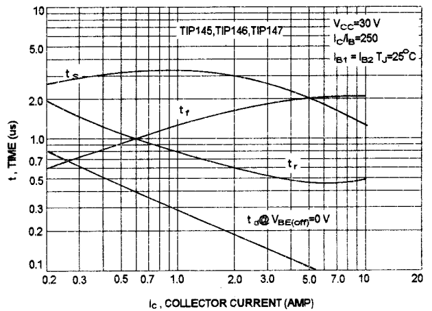
SWITCHING TIME
