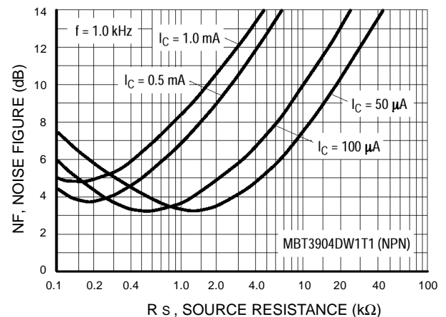
Figure 10. Noise Figure
