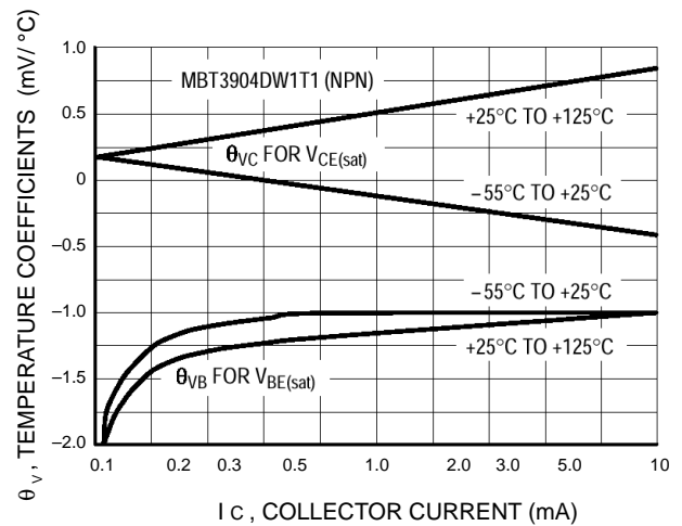
Figure 18. Temperature Coefficients
