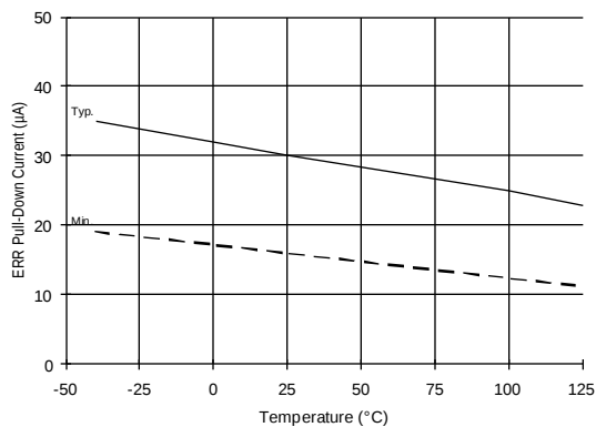
Figure 29A. ERR Pull-Down Current vs. Temperature
