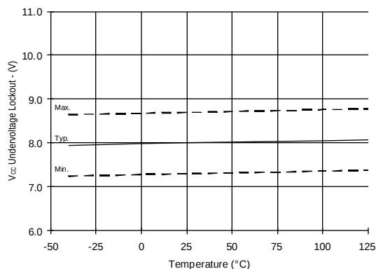
Figure 26. V_{CC} Undervoltage (-) vs. Temperature
