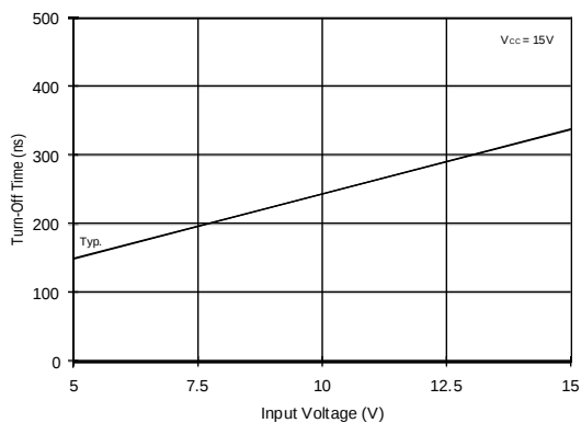
Figure 32B. Turn-Off Time vs. Input Voltage
