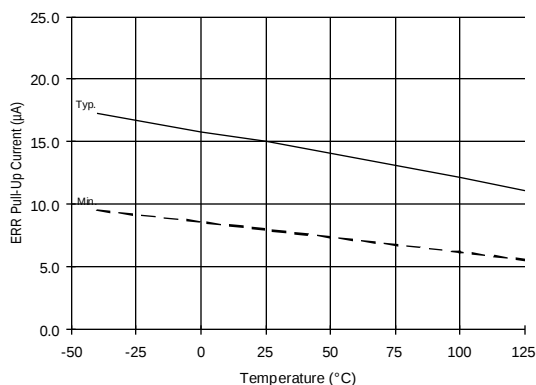
Figure 28A. ERR Pull-Up Current vs. Temperature
