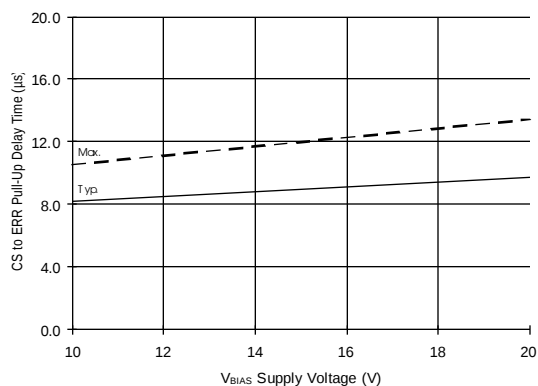
Figure 13B. CS to ERR Pull-Up vs. Voltage
