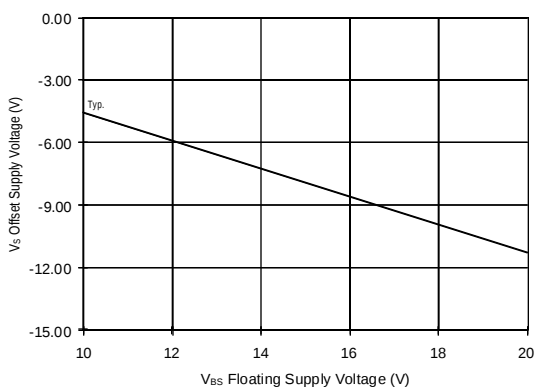
Figure 33. Maximum V_S Negative Offset vs. Supply Voltage
