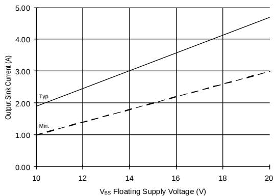
Figure 31B. Output Sink Current vs. Voltage
