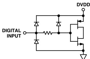
Figure 28. Equivalent Digital Input
