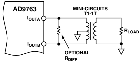
Figure 33. Differential Output Using a Transformer
