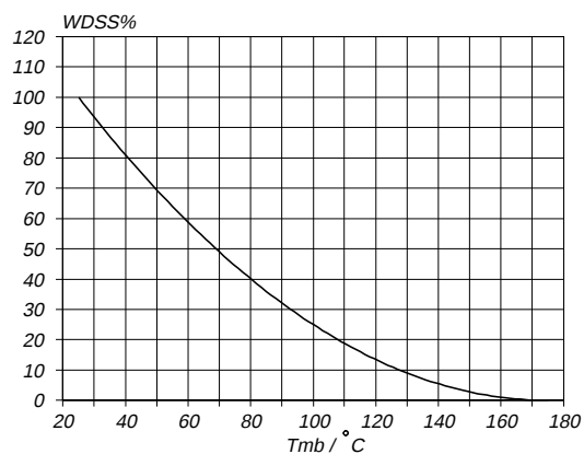
Fig.15. Normalised avalanche energy rating. W_{DSS}\% = f(T_{mb}) ; conditions: I_D = 22\text{ A}
