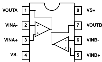
EL2227 (8-PIN SO, MSOP) TOP VIEW
