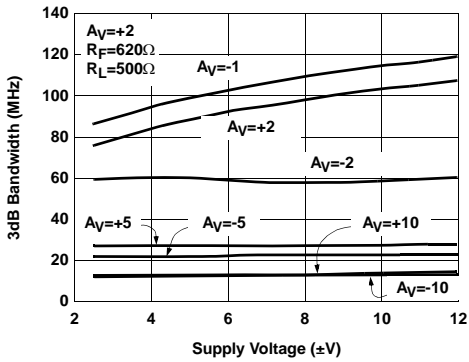
3dB Bandwidth vs Supply Voltage
