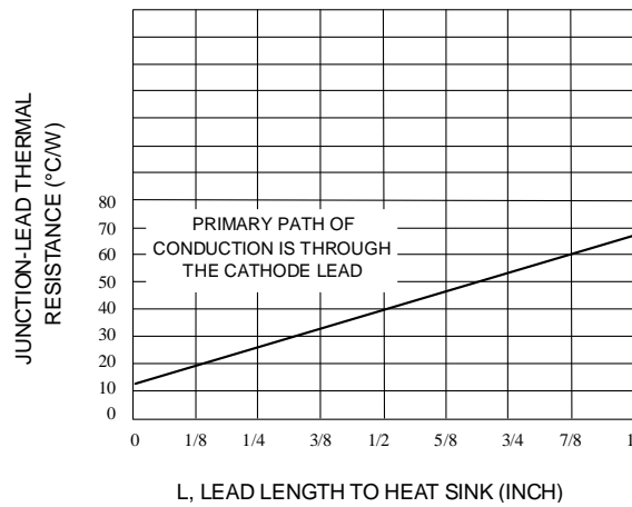
Fig. 9 -TYPICAL THERMAL RESISTANCE
