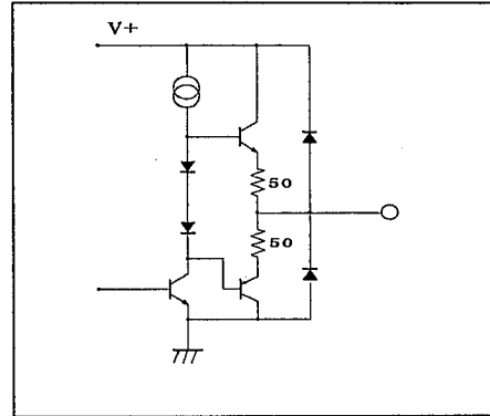
4, 7, 8, 9, 10, 11, 12, 15, 17, 21, 28 PIN
