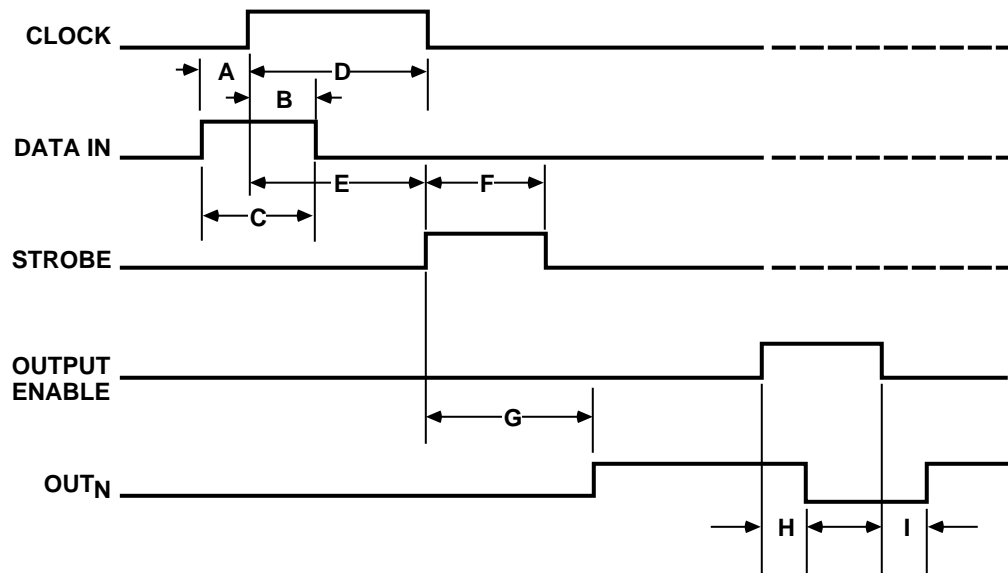
Timing Conditions
