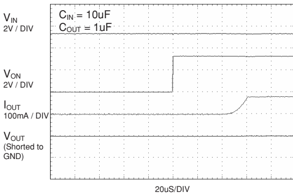
Figure 19. Current-Limit Response Time (Output to GND)
