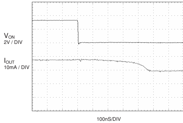
Figure 16. Turn-Off Response
