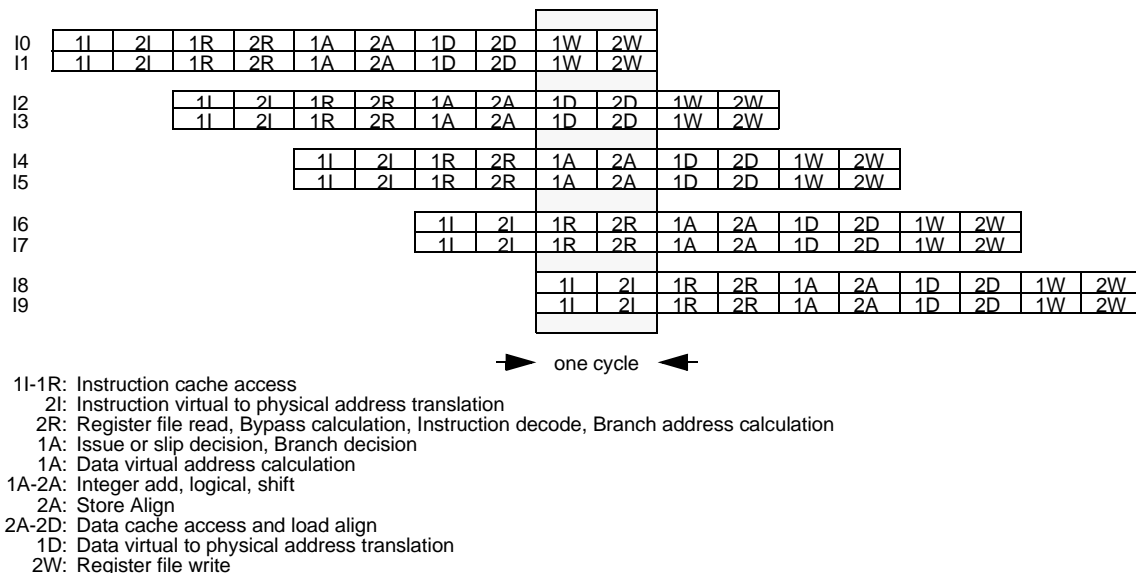
Figure 4 Pipeline
