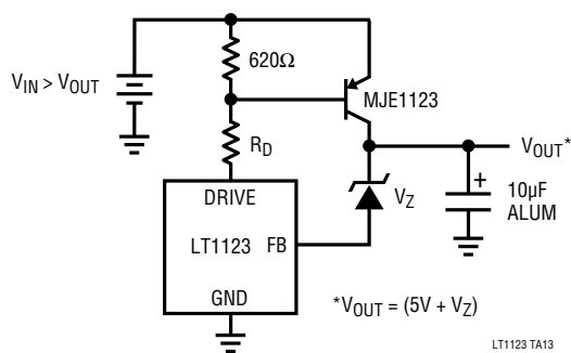
Adjusting V_{OUT}
