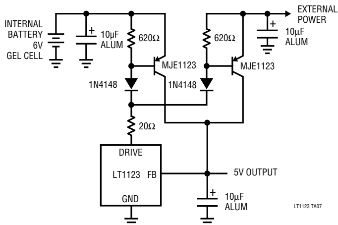
Battery Backup Regulator
