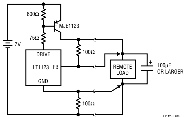
5V/2A Regulator with Remote Sensing
