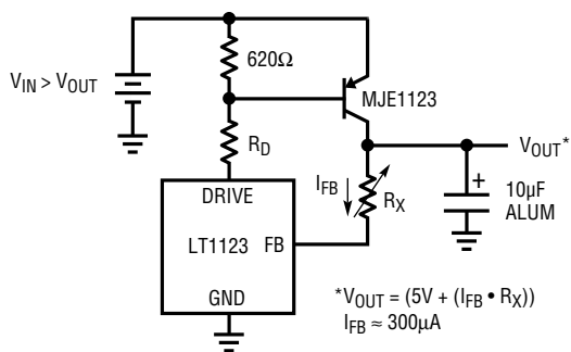
Adjusting V_{OUT}
